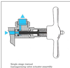
Single-stage manual homogenizing valve actuator assembly
