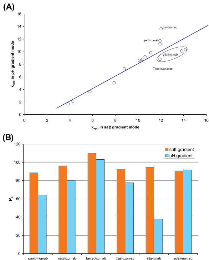
Fig. 8. Comparison of retention factors (A) and peak capacity (B) in salt and pH gradient mode cation exchange chromatography. Conditions as defined in the legend of Fig. 7 for the pH gradient, and as defined in Ref. [24] for the generic salt gradient.
