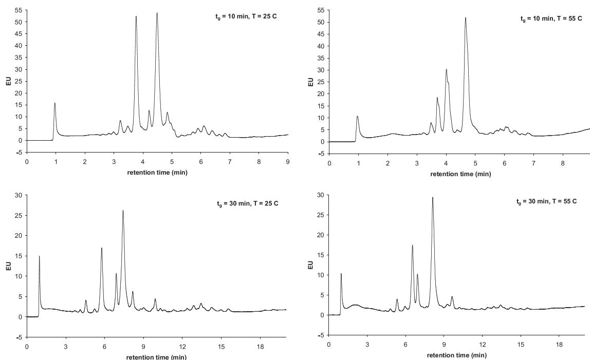
Fig. 4. Cetuximab papain digested sample. Column: YMC BioPro SP-F (100 mm × 4.6 mm). Mobile phase “A” CX-1 Buffer A pH 5.6, “B” CX-1 Buffer B pH 10.2. Flow rate: 0.6 ml/min, gradient: 0–80%B, detection: FL (280–360 nm), injected volume: 2 \mu l. Gradient times: t_{g1} = 10 min, t_{g2} = 30 min, temperatures T_1 = 25 °C, T_2 = 55 °C.
