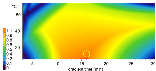
Fig. 5. Cetuximab papain digestion resolution map ( t_g - T model). Column: YMC BioPro SP-F (100 mm × 4.6 mm). Mobile phase “A” CX-1 Buffer A pH 5.6, “B” CX-1 Buffer B pH 10.2. Flow rate: 0.6 ml/min, gradient: 0–80%B, detection: FL (280–360 nm), injected volume: 2 \mu l. Gradient times: t_{g1} = 10 min, t_{g2} = 30 min, temperatures T_1 = 25 °C, T_2 = 55 °C.
