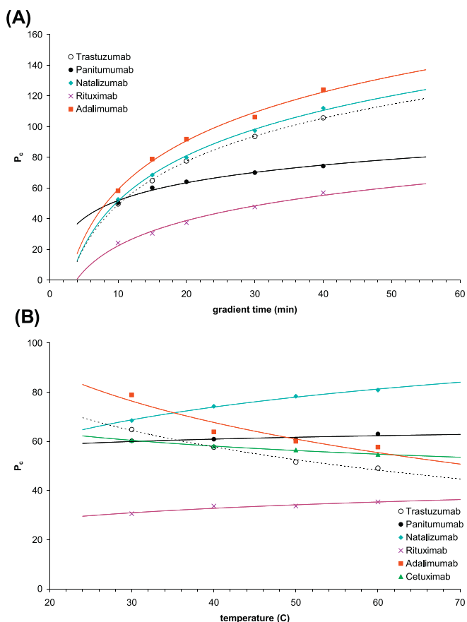
Fig. 3. Peak capacity as a function of gradient time (steepness) (A) and temperature (B). Column: YMC BioPro SP-F (100 mm × 4.6 mm). Mobile phase "A" CX-1 Buffer A pH 5.6, "B" CX-1 Buffer B pH 10.2. Flow rate: 0.6 ml/min, detection: FL (280–360 nm), injected volume: 2 \mu l.
