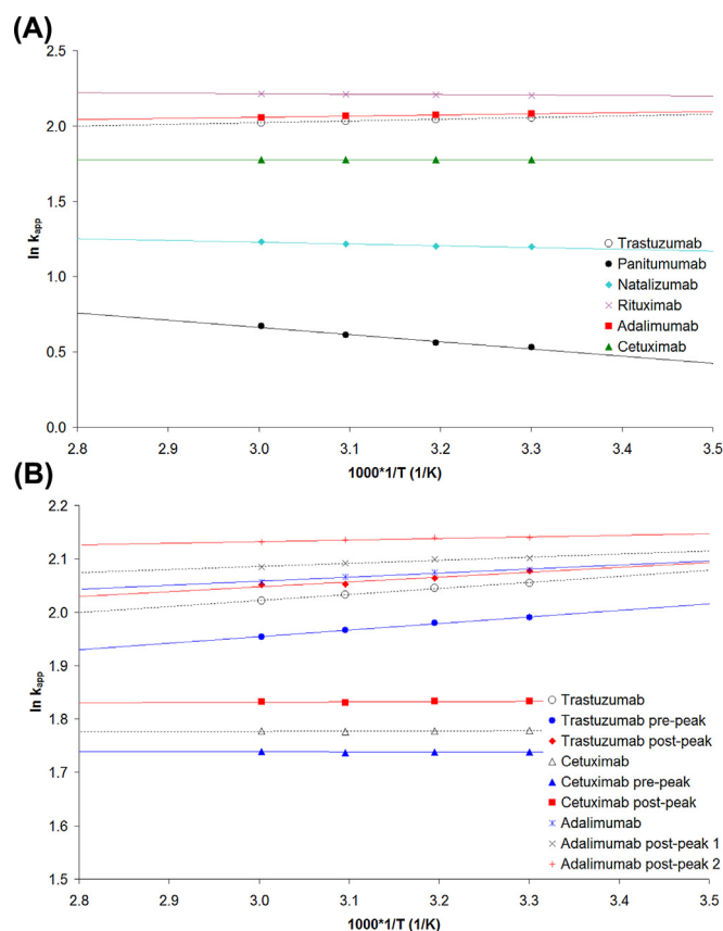
Fig. 2. Effect of temperature on the apparent retention factor of native antibodies (A) and antibody variants (B) (van't Hoff type representation). Column: YMC BioPro SP-F (100 mm \times 4.6 mm). Mobile phase "A" CX-1 Buffer A pH 5.6, "B" CX-1 Buffer B pH 10.2. Flow rate: 0.6 ml/min, gradient: 0–100%B in 15 min, temperature: 30, 40, 50 and 60 °C, detection: FL (280–360 nm), injected volume: 2 \mu l.
