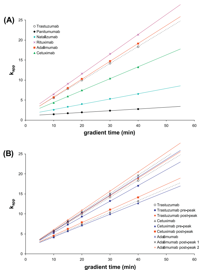
Fig. 1. Effect of gradient time (steepness) on the apparent retention factor of native antibodies (A) and antibody variants (B). Column: YMC BioPro SP-F (100 mm \times 4.6 mm). Mobile phase "A" CX-1 Buffer A pH 5.6, "B" CX-1 Buffer B pH 10.2. Flow rate: 0.6 ml/min, gradient: 0–100%B in 10, 15, 20, 30 and 40 min, temperature: 30 °C, detection: FL (280–360 nm), injected volume: 2 \mu l.
