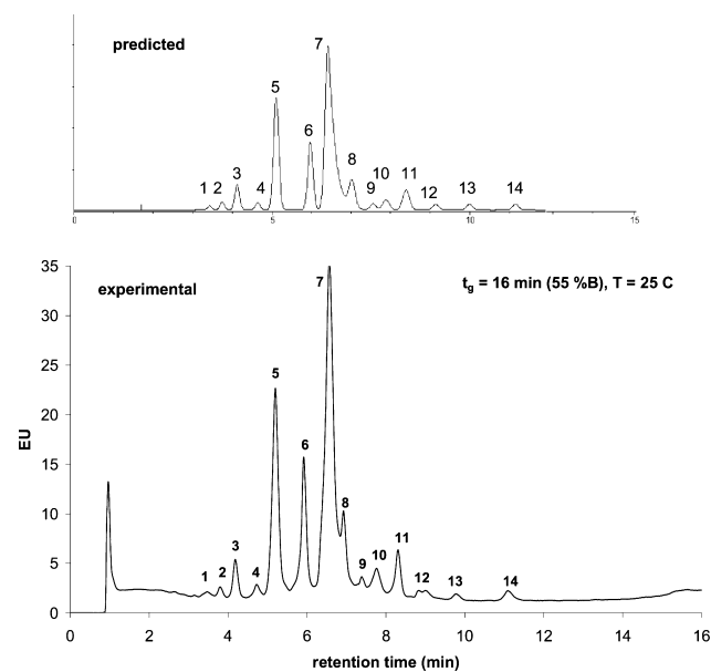
Fig. 6. Comparison of predicted and experimental chromatograms. Column: YMC BioPro SP-F (100 mm × 4.6 mm). Mobile phase “A” CX-1 Buffer A pH 5.6, “B” CX-1 Buffer B pH 10.2. Flow rate: 0.6 ml/min, gradient: 0–55%B in 16 min, temperature: 25 °C, detection: FL (280–360 nm), injected volume: 2 \mu l.
