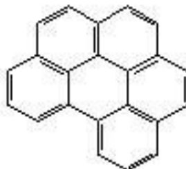
Benzo[g,h,j]perylene
