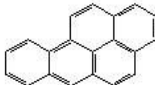
Benzo[a]pyrene
